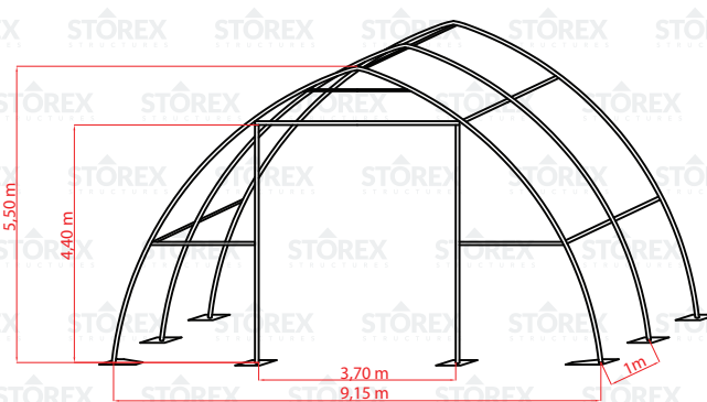
Partial 3D drawing (not all frame arches are shown)
