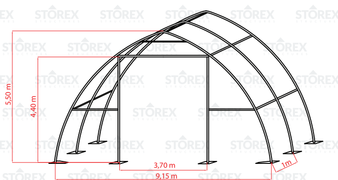
Partial 3D drawing (not all frame arches are shown)
