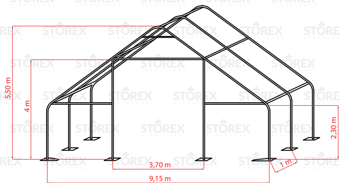
Partial 3D drawing (not all frame arches are shown)
